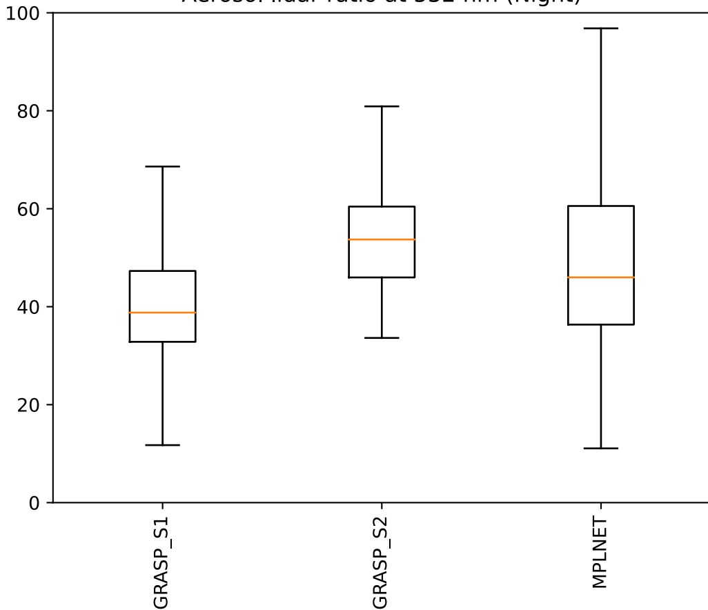
Aerosol lidar ratio at 532 nm (Night)
